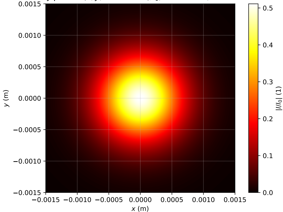
Intensity profile I(x, y, z = 3.264m)/I_0 , Pin=0.5Pcr, artificial time
